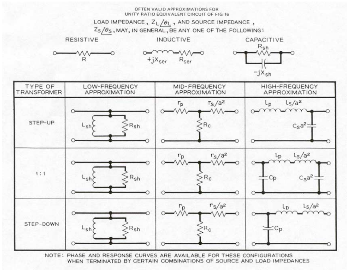
Figure 16—Often valid approximations for equivalent circuit of Figure 6
