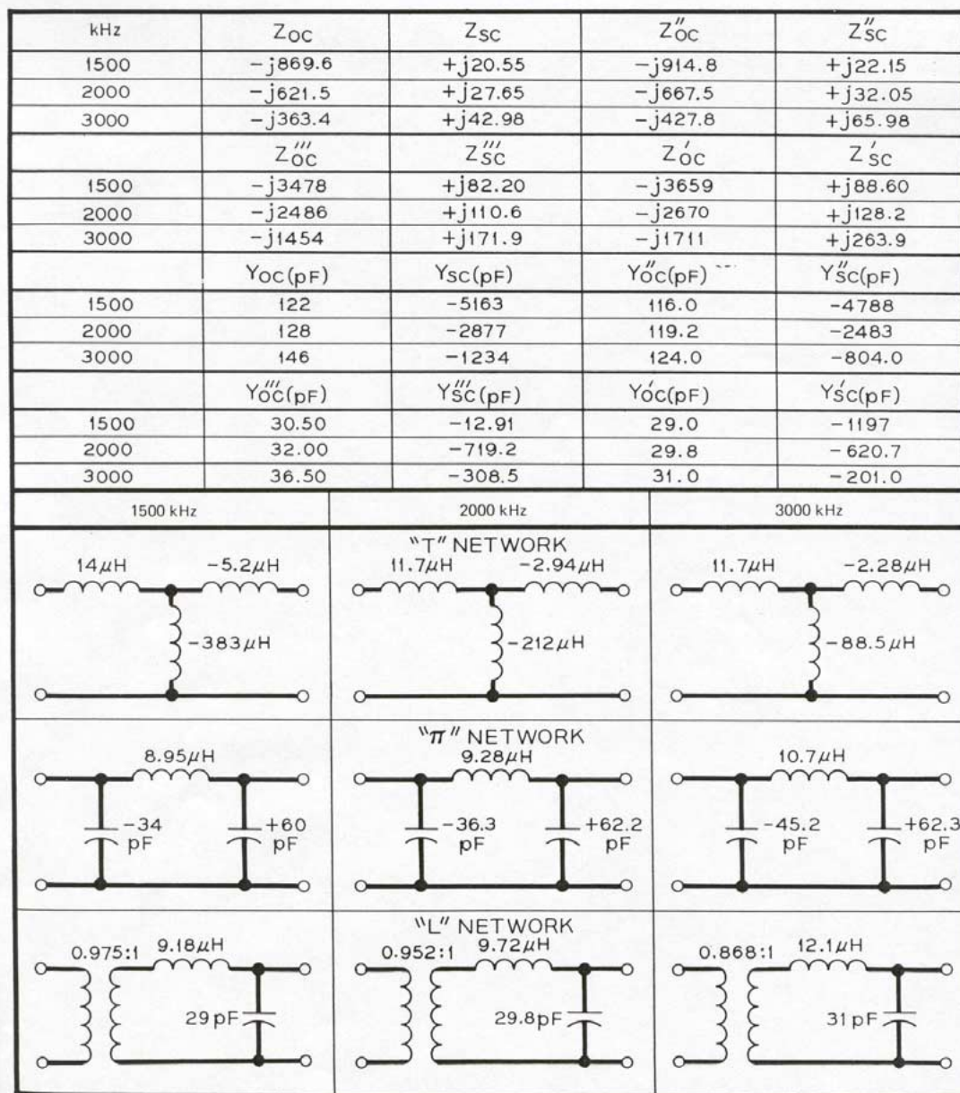
Figure 17—Impedance characteristics of transformers used in examples
