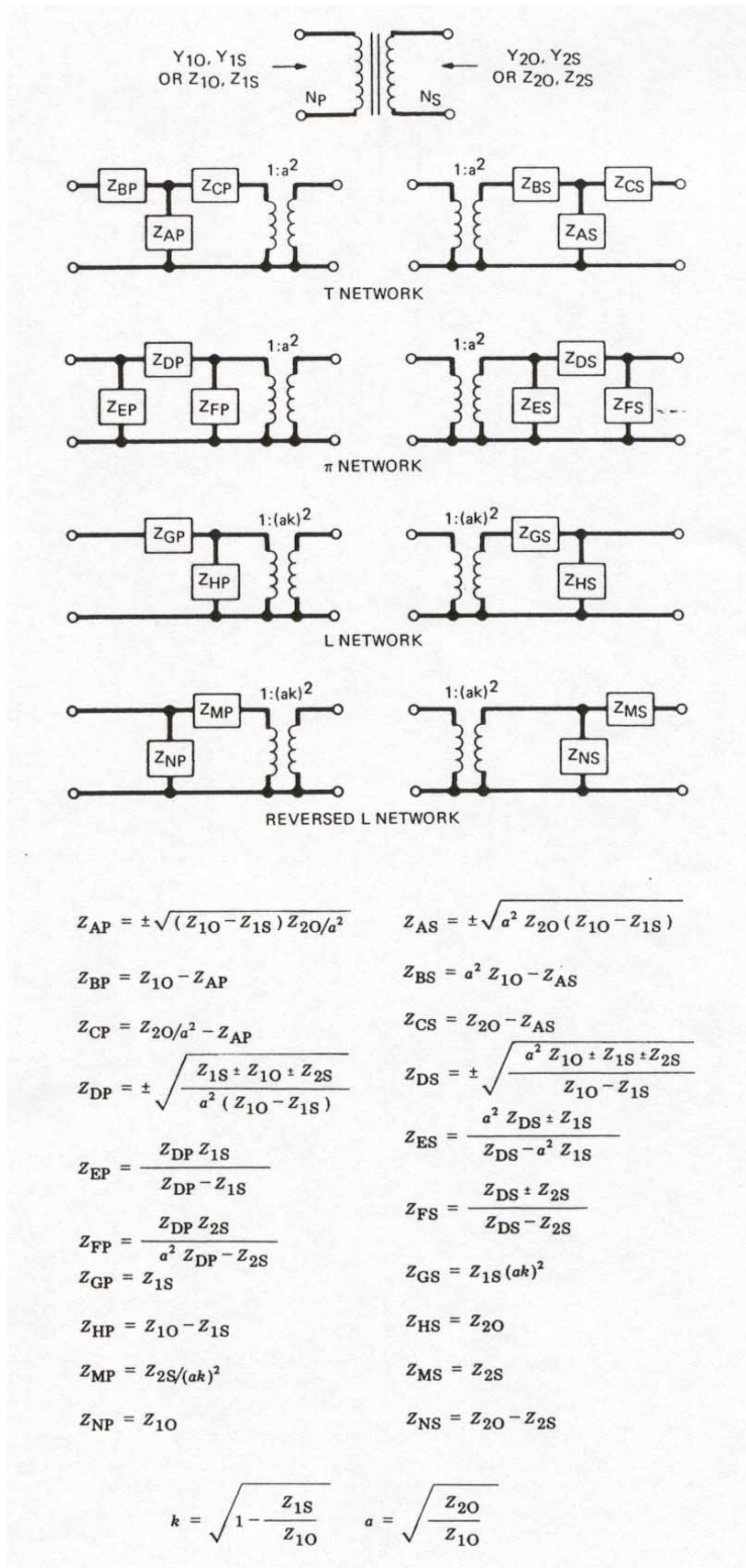
Figure 15—Three-terminal equivalent networks determined from open- and short-circuit measurements
