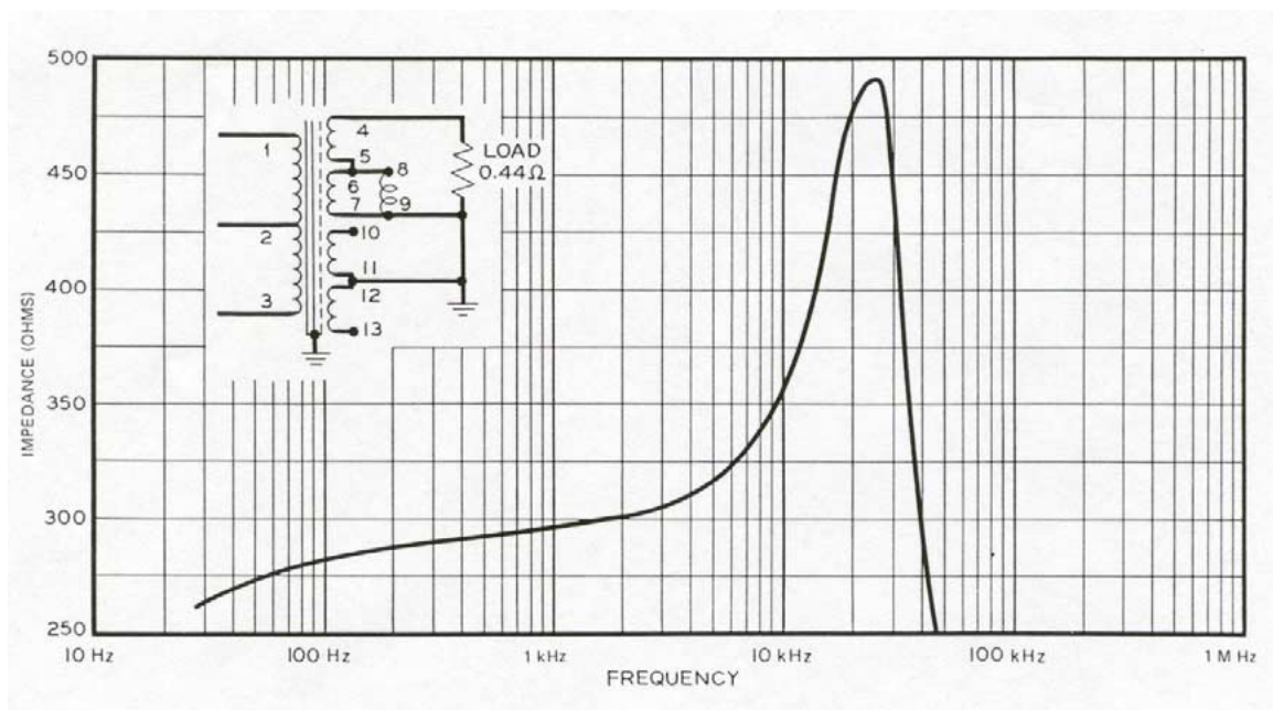
Figure 11—Example of the impedance of windings (1-3) with windings (4-7) terminated
