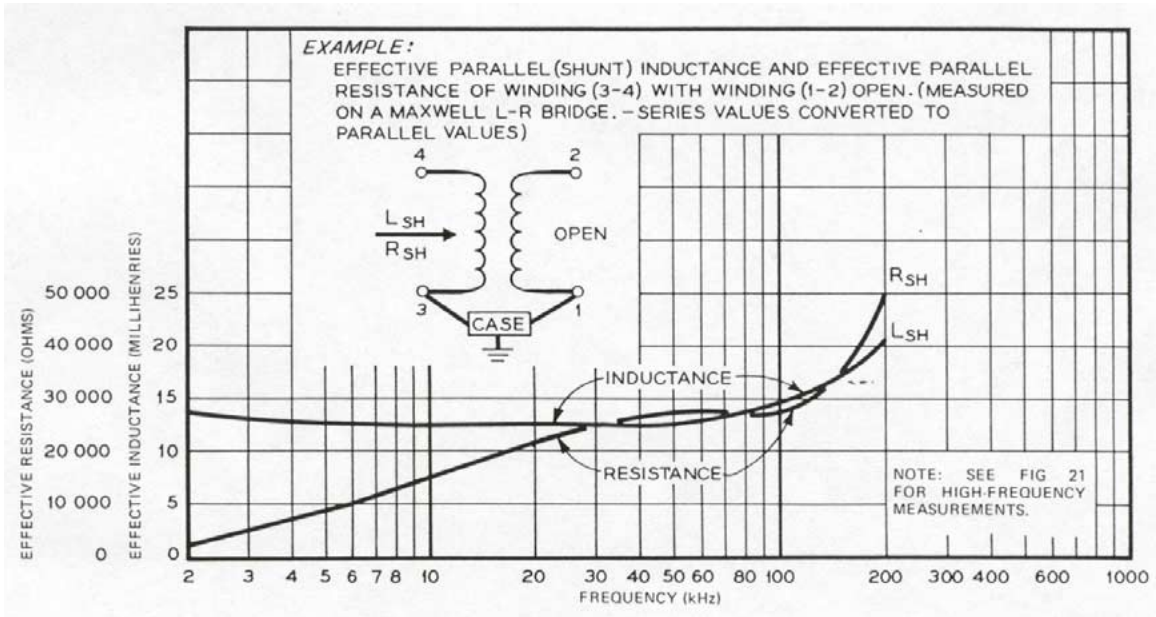
Figure 20—Example of an effective parallel inductance and resistance of winding (3-4) with winding (1-2) open
