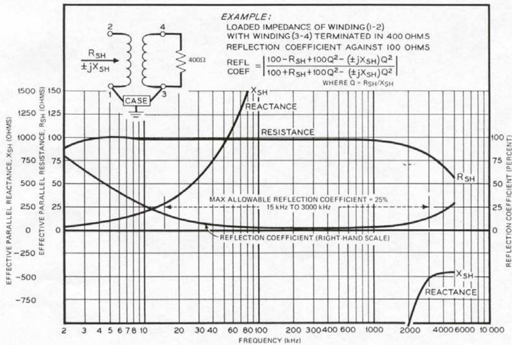
Figure 13—Example of loaded impedance and reflection coefficient curves for a fictitious transformer
