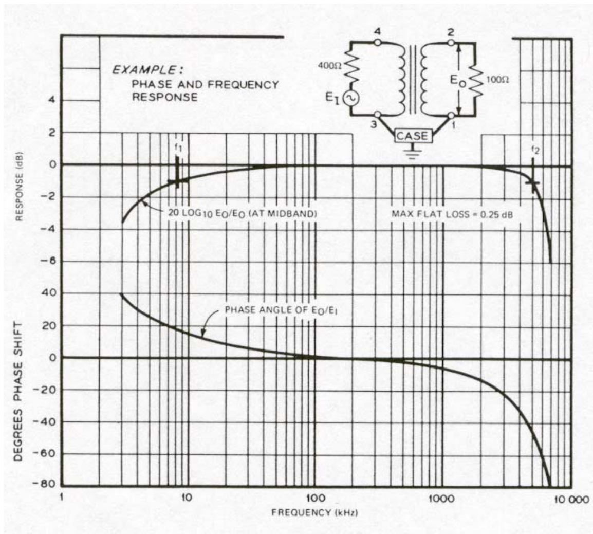
Figure 5—Example of phase and frequency response
