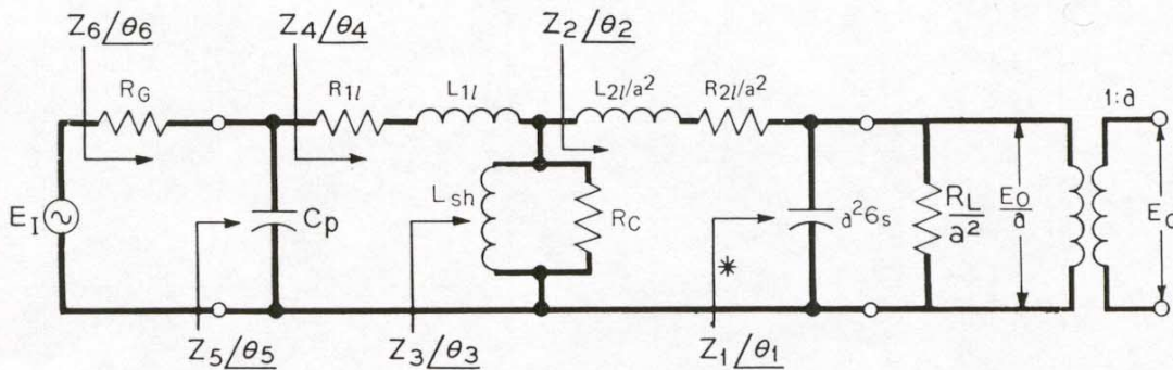
Equivalent circuit
