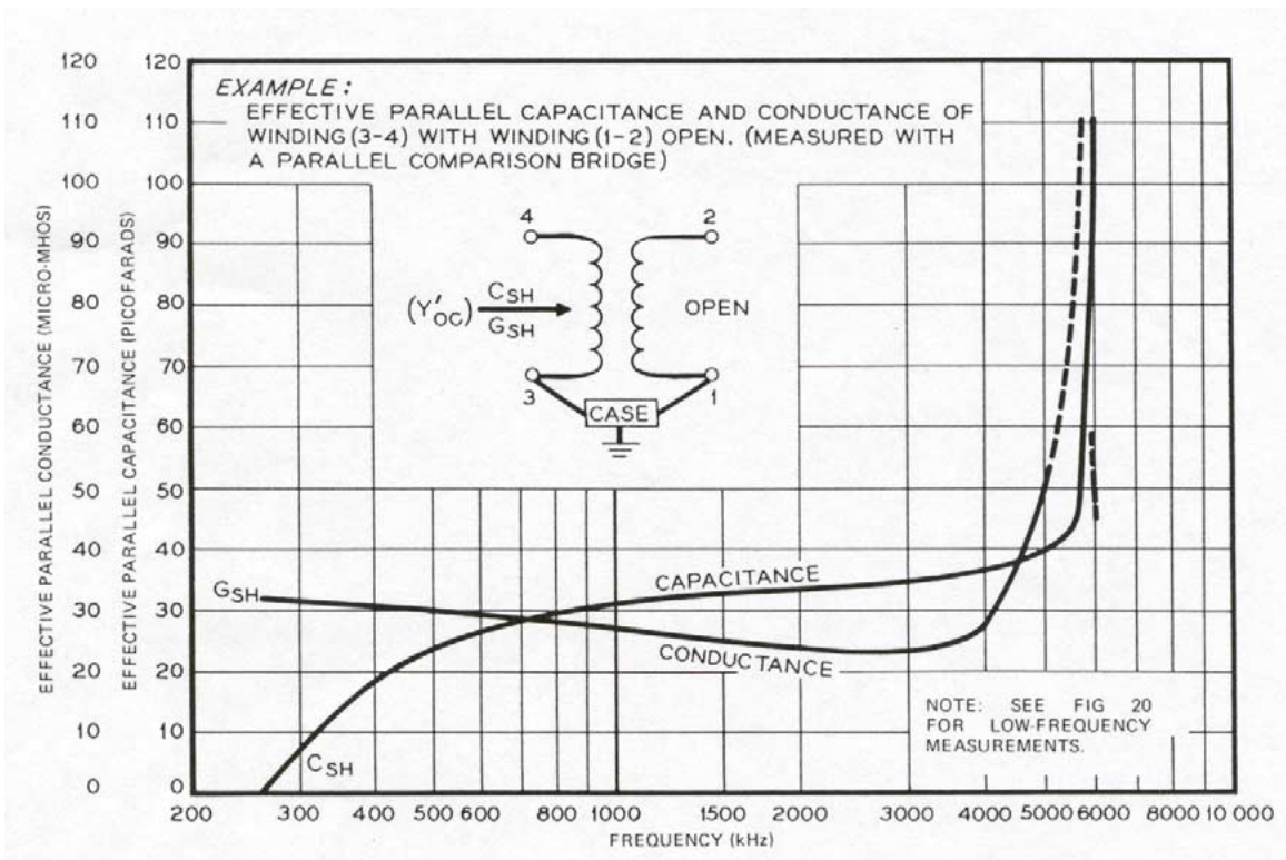
Figure 21—Example of an effective parallel capacitance and conductance of winding (3-4) with winding (1-2) open
