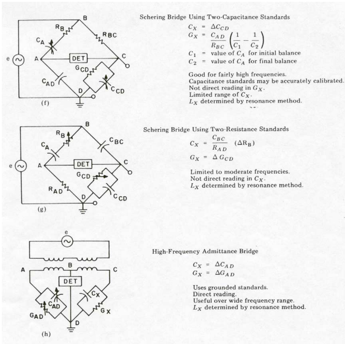
Figure 22—Impedance bridges (continued)
