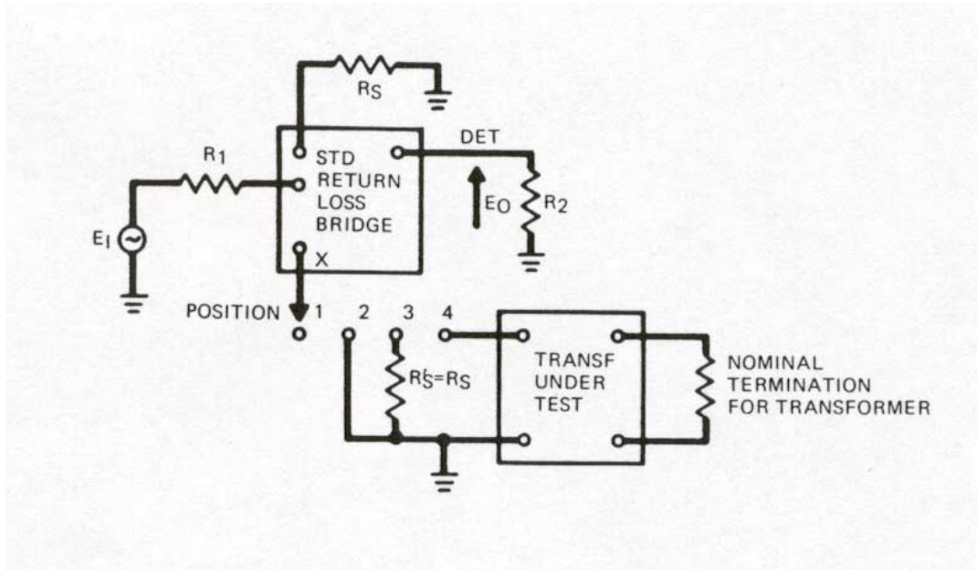
Figure 24—Return loss measurement
