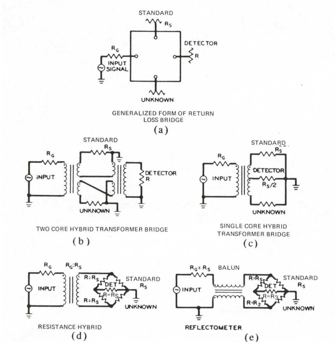
Figure 23—Return loss bridge
