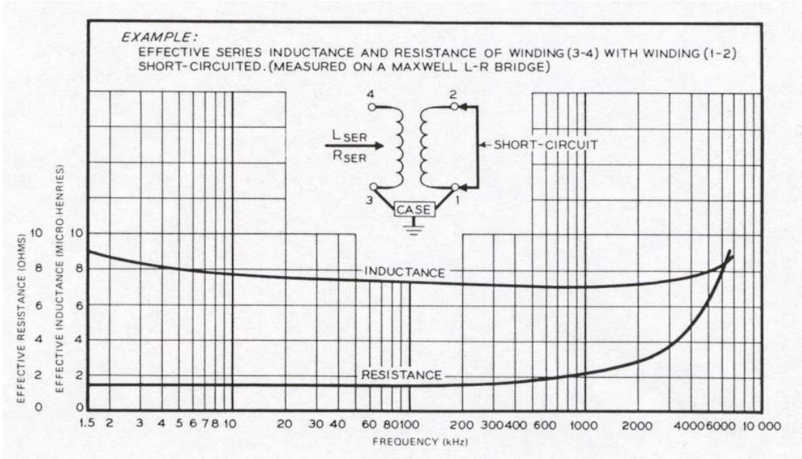
Figure 3—Example of an effective series inductance and resistance of winding (3-4) with winding (1-2) short-circuited
