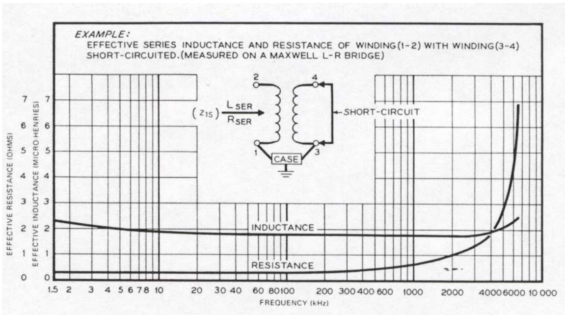
Figure 2—Example of an effective series inductance and resistance of winding (1-2) with winding (3-4) short-circuited
