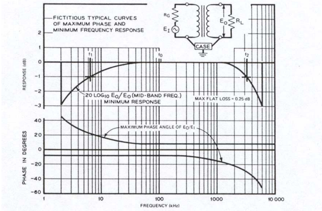
Figure 8—Fictitious typical curves of maximum phase and minimum frequency response
