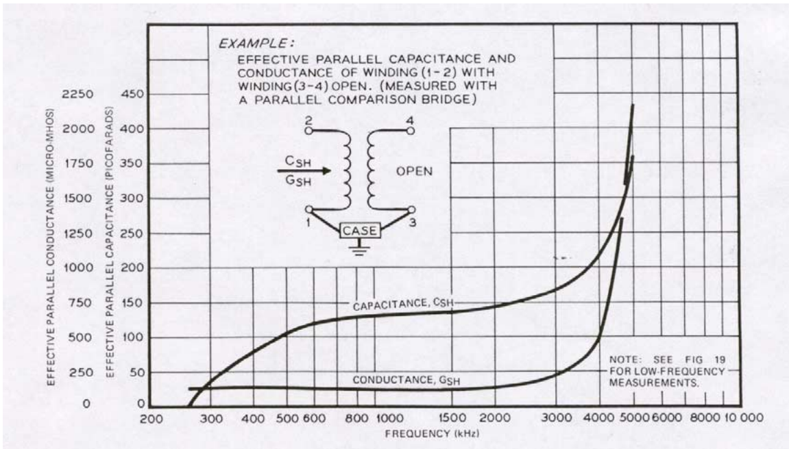
Figure 18—Example of an effective parallel capacitance and conductance of winding (1-2) with winding (3-4) open
