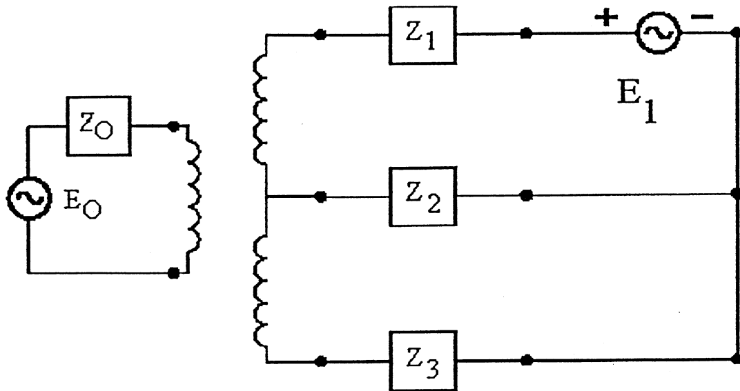
Figure 25—Hybrid transformer
