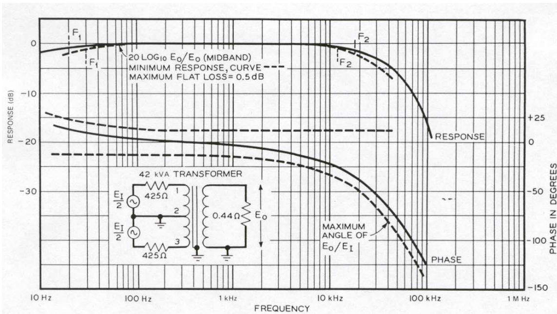
Figure 4—Example of the response of a transformer with matched resistive terminations and typical curves of maximum phase and minimum frequency response
