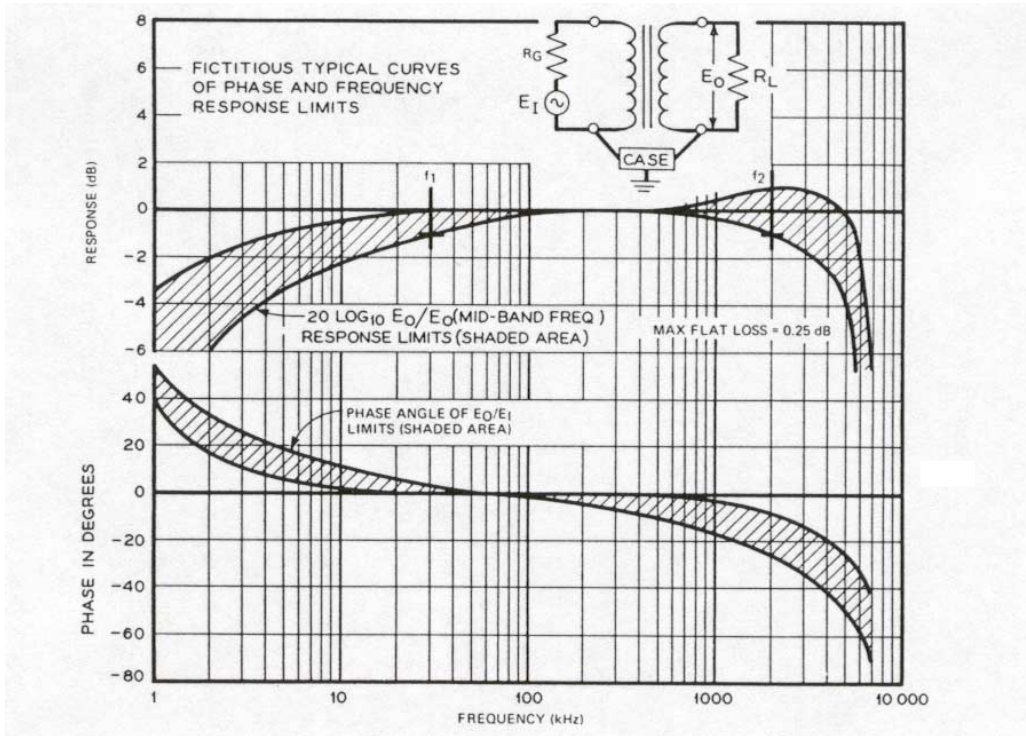
Figure 7—Fictitious typical curves of phase and frequency response limits
