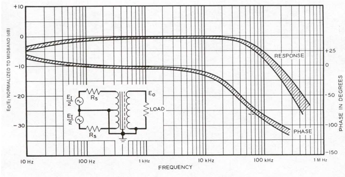
Figure 9—Example of the tolerance band of the response of a transformer with matched resistive termination
