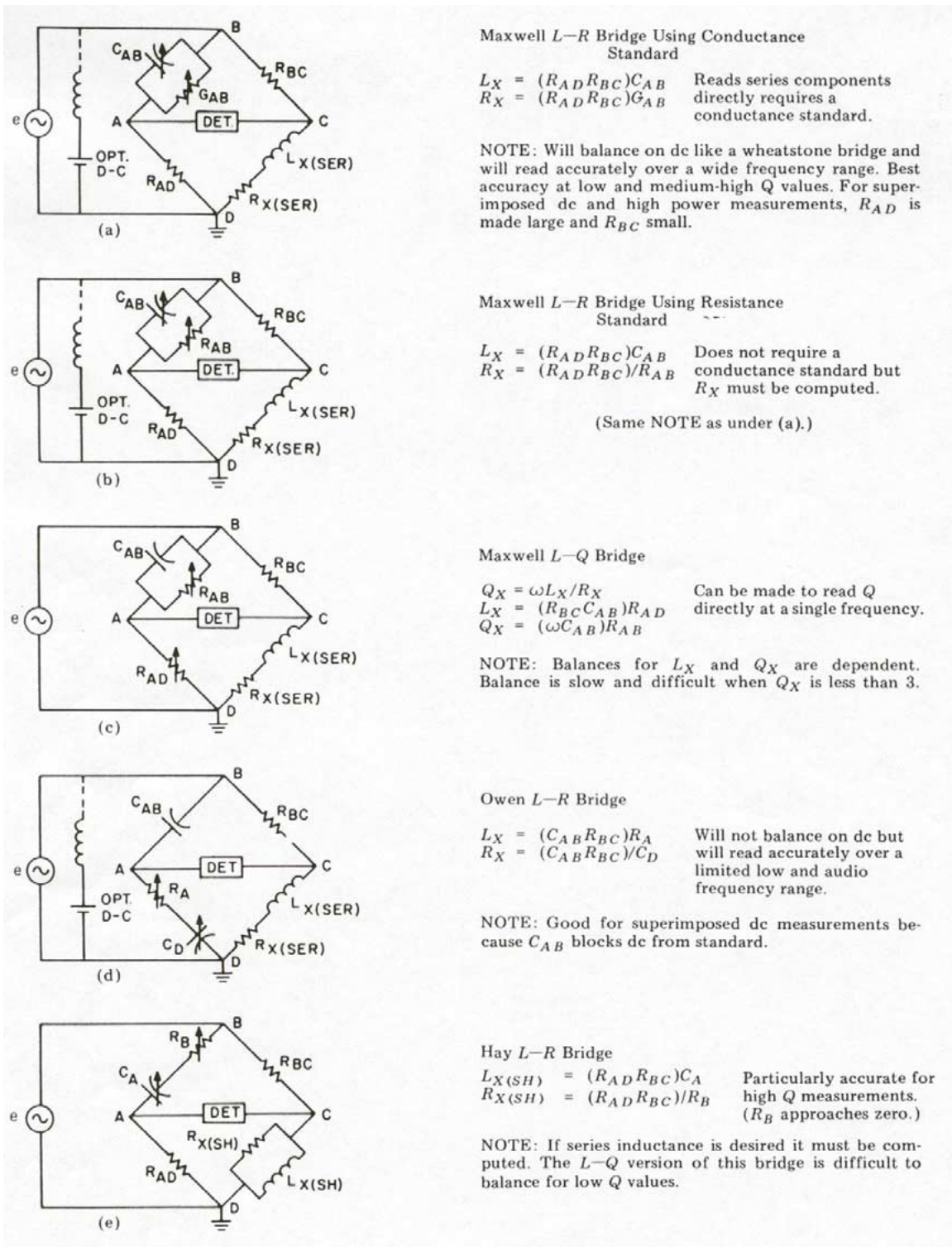
Figure 22—Impedance bridge
