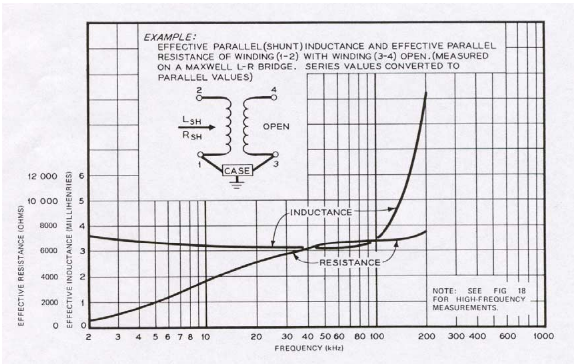
Figure 19—Example of effective parallel inductance and resistance of winding (1-2) with winding (3-4) open
