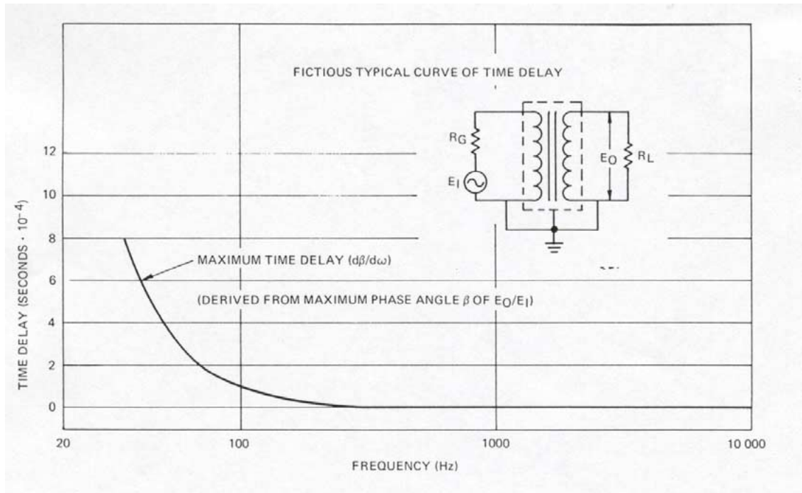
Figure 10—Fictitious typical curve of time delay
