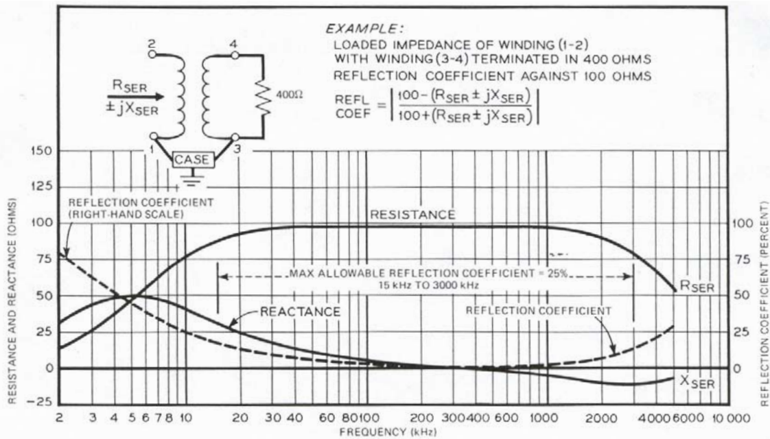
Figure 12—Example of return-loss resistance and reflection coefficient curves for a fictitious transformer
