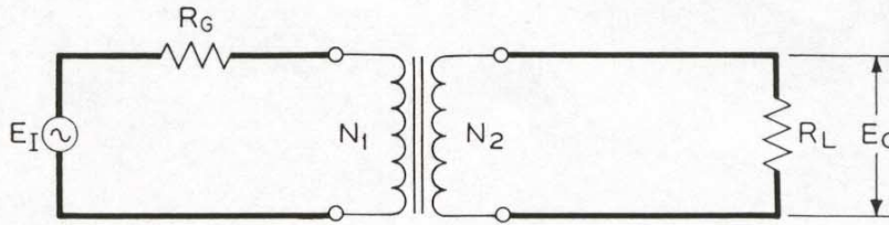
Transformer equivalent circuit
